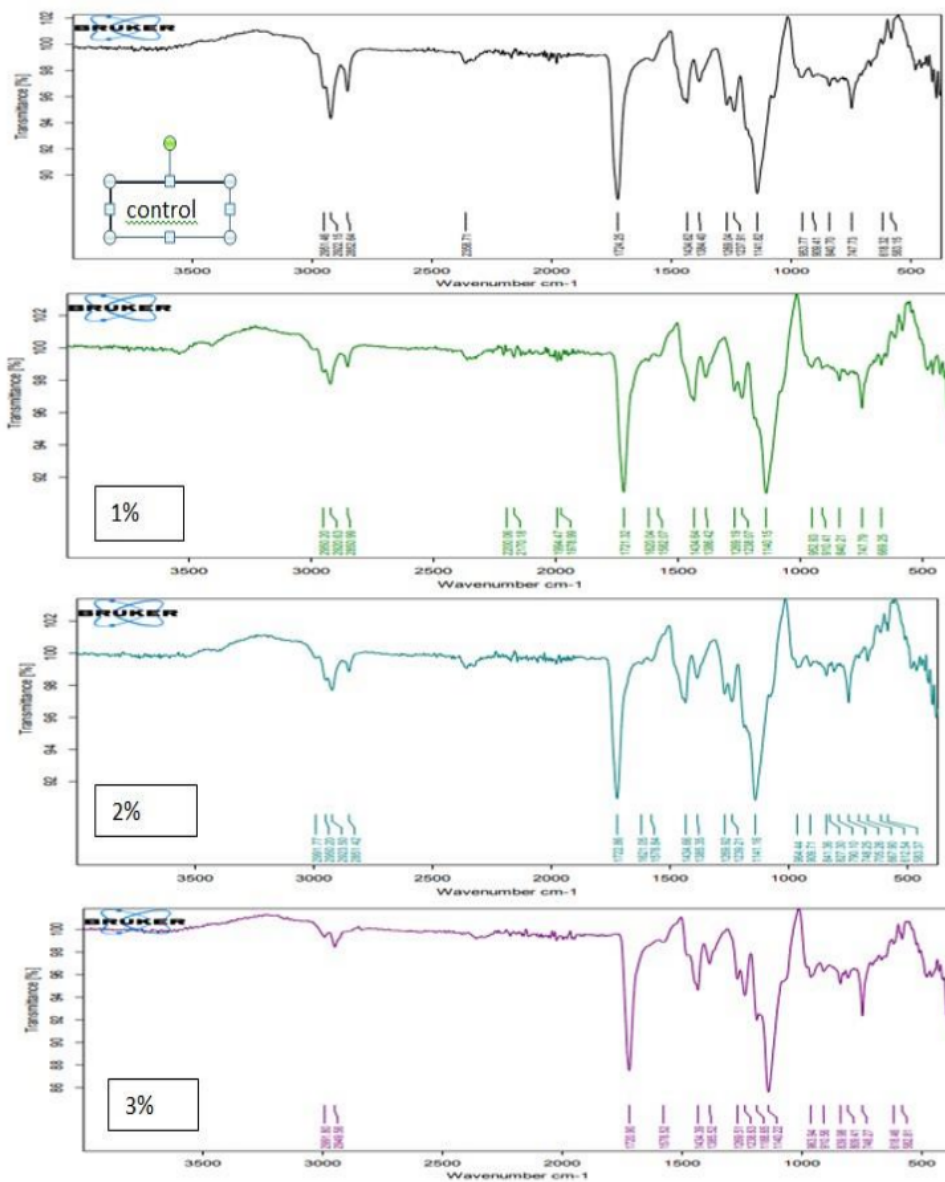
Figure 2: FTAR shows there is no chemical change in the properties of the substance between nature coconut oil and heat cure resin in different concentrations of oil.
