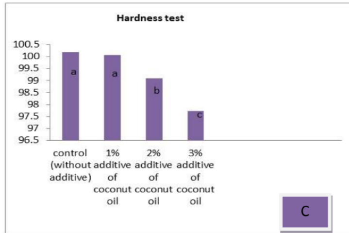
Figure 3 : Mean value of three additive groups (1%, 2%, and 3%) and control group for: A. adherence cell of candida albican test , B. flexural strength test, C. hardness test.
