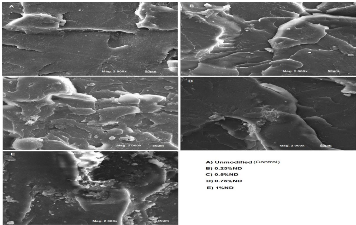
Figure 4 (A-E): Representative SEM image for fractured surfaces. A) Unmodified specimens. B) 0.25%ND, C) 0.5%ND, D) 0.75%ND, E) 1%ND.
