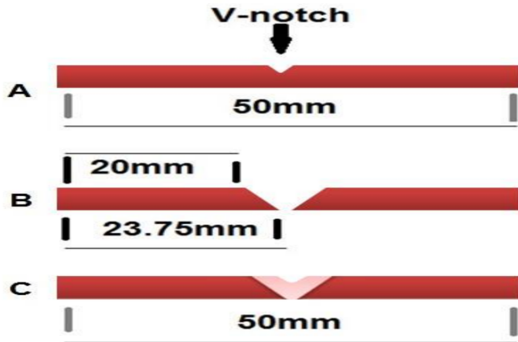
3 Figure 1 A-C: Schematic diagram for acrylic resin specimen's dimensions and preparation. A) Intact specimen, B) prepared specimen for repair, C) repaired specimens.
