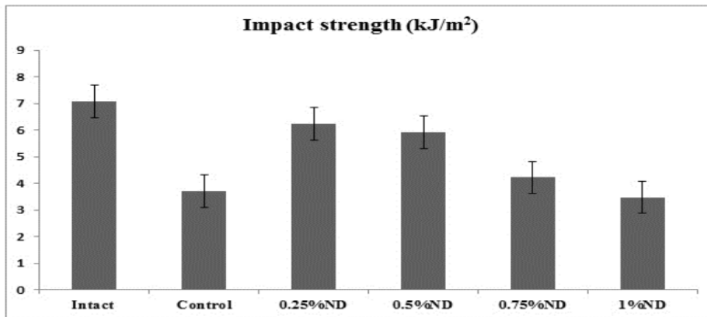
9 Figure 3: Mean value of impact strength for all tested groups.
